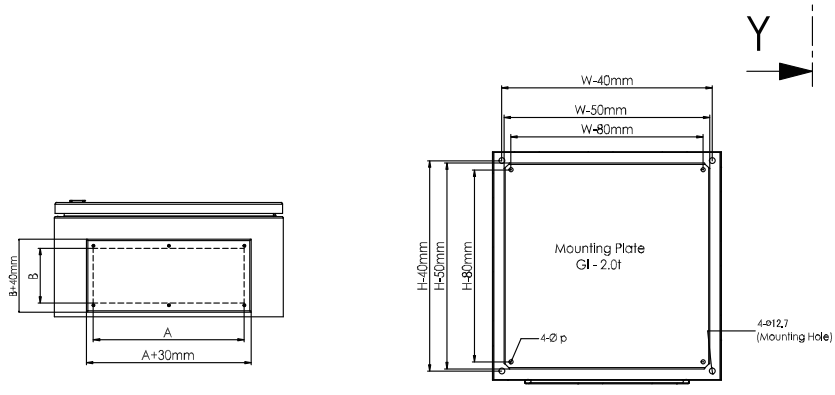
Section View Y-Y
