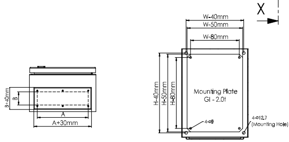
Section View X-X
